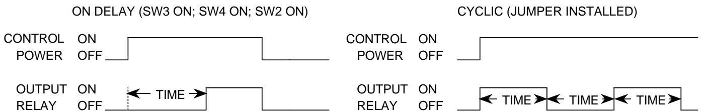
FIG. 4: TIMING LOGIC CHARTS
